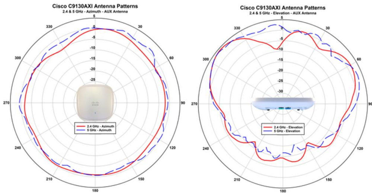
Figure 24. Cisco Catalyst 9130I antenna patterns, RF ASIC (AUX dual band)
