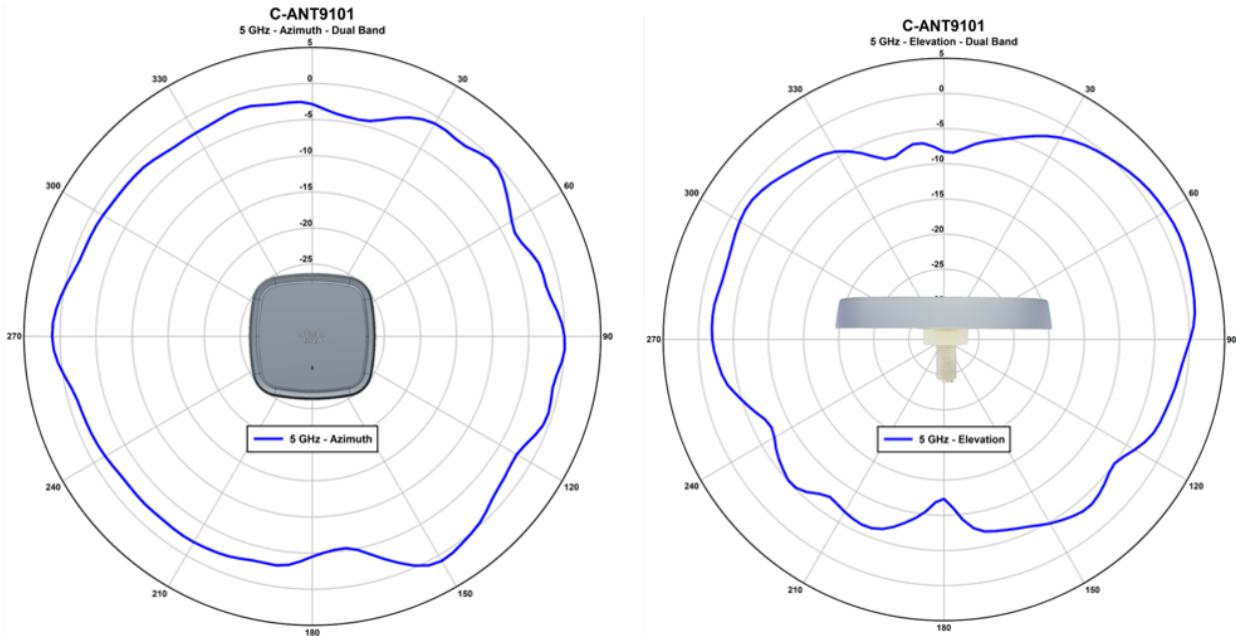
Figure 35. C-ANT9101 antenna patterns, 5-GHz dual band
