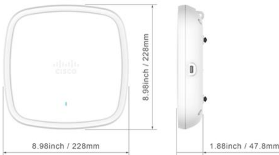
Figure 2. Mechanicals: 9130I model
