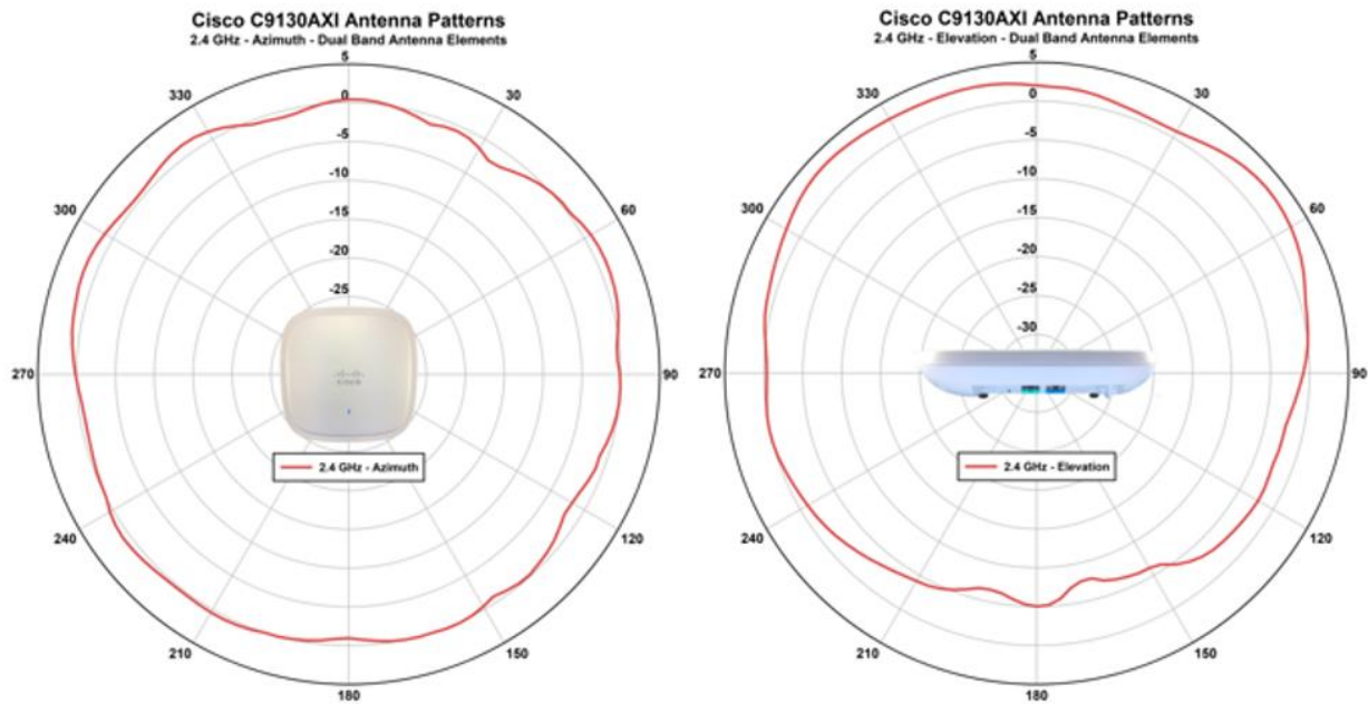
Figure 23. Cisco Catalyst 9130I antenna patterns, dual-band 2.4 GHz
