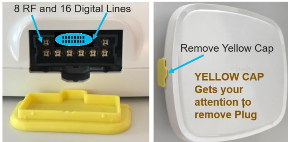
Figure 27. 9130E antenna connector details
