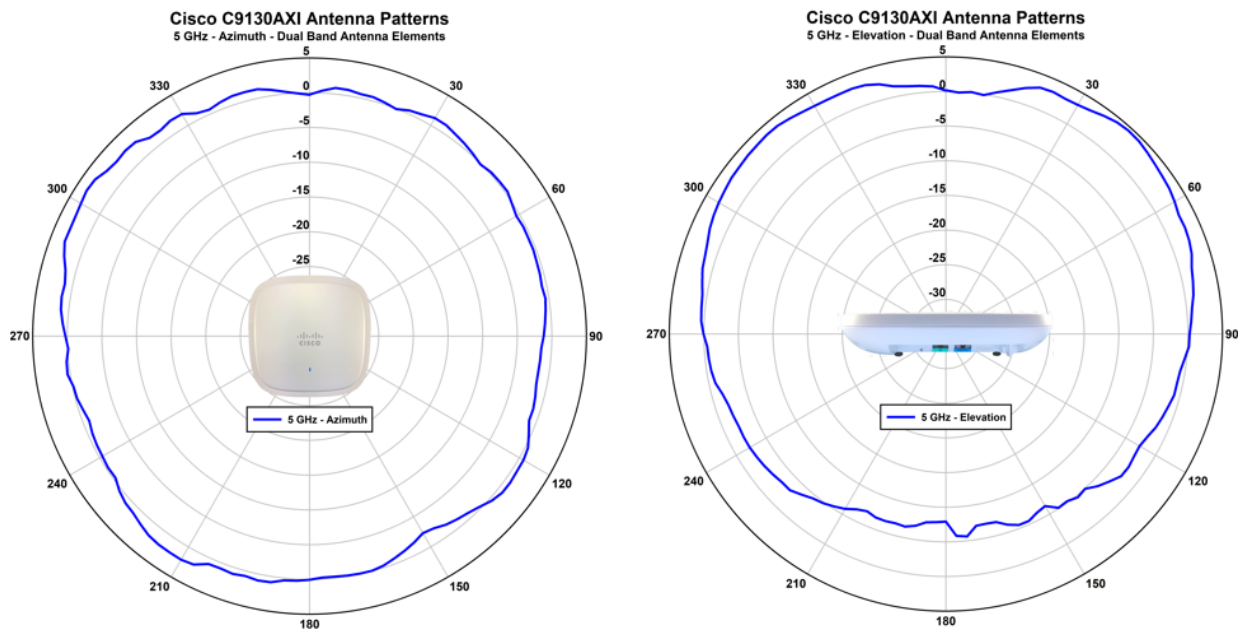
Figure 21. Cisco Catalyst 9130I antenna patterns, dual-band 5 GHz
