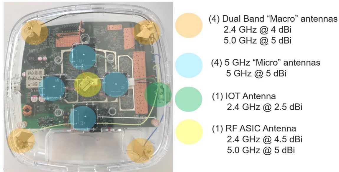
Figure 19. 9130I internal antenna system
